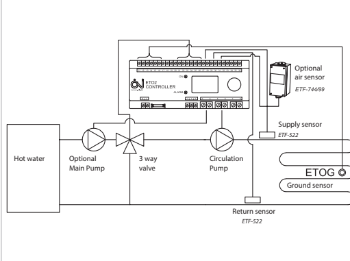
Example: Advanced 1-zone hydronic application
