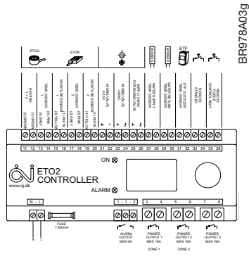
Connections
