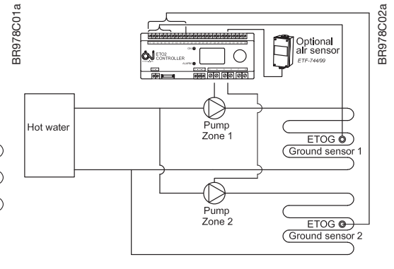
Example: Simple 2-zone hydronic application
