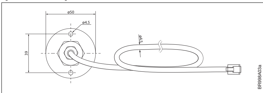
Fig. 5 Dimensioned drawing
