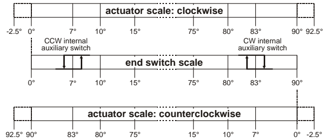
Fig. 4. Internal end switch triggering points
