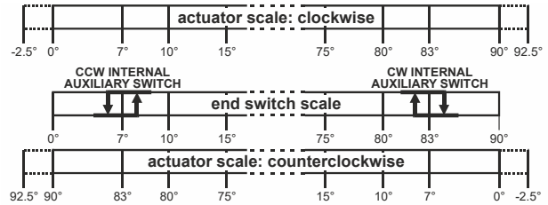
Fig. 4. Internal end switch triggering points
