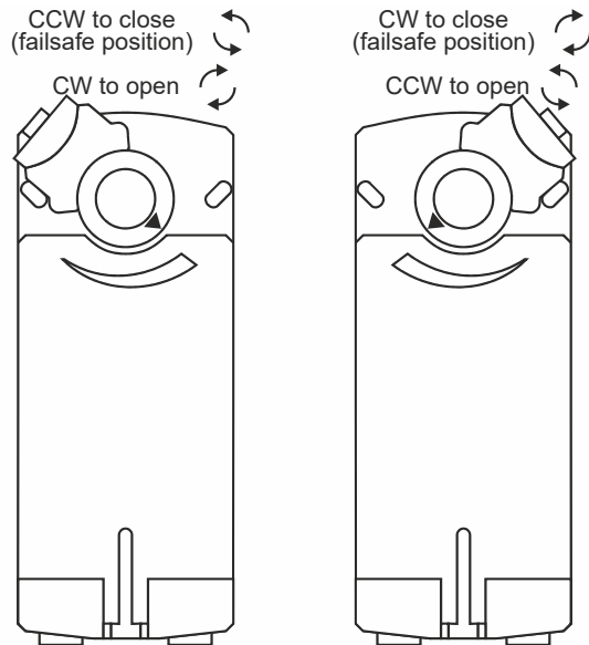
Fig. 2. Mounting orientation
