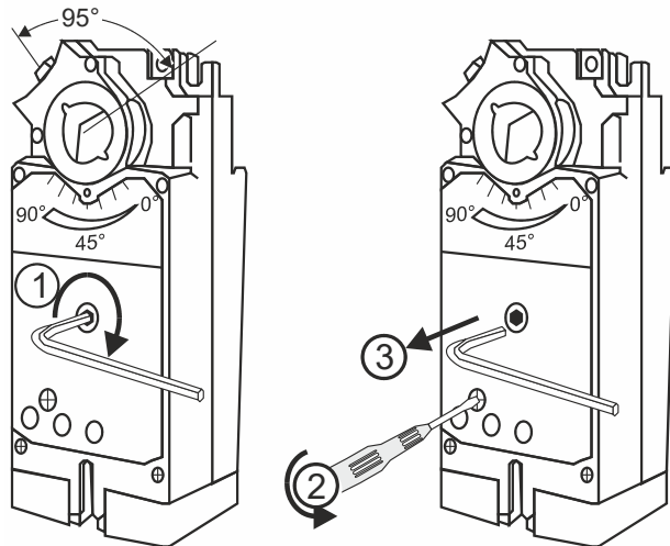
Fig. 3. Manual positioning
