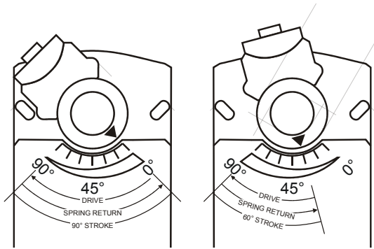
Fig. 5. Stroke reduction
