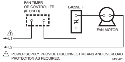
Fig. 5. Typical diagram of L4029E or F in ventilating fan circuit.
