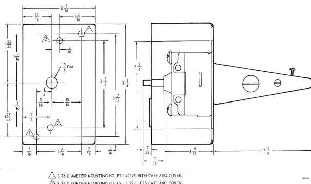
Fig. 2. Control dimensions.
