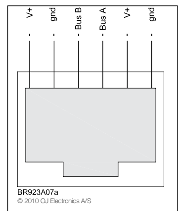
Fig. 3 Modbus connection
