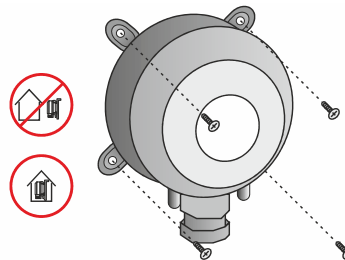
Fig. 2. Mounting
