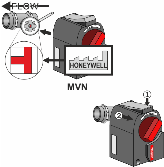
7: TWO- AND THREE-WAY VALVES (DN15...32)
