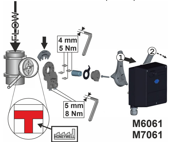
8: TWO- AND THREE-WAY VALVES (DN40-50)
